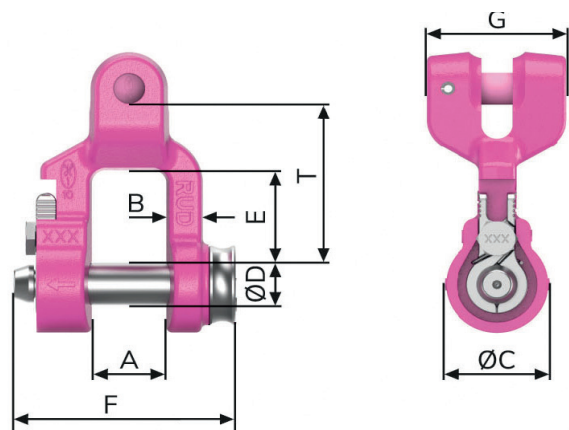
Pic. 29: VIP CCS-FASTLOX 6-22 mm
