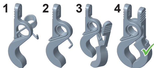
Pic. 24: Assembly sequence of leg spring
