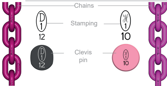
Pic. 4: Difference between ICE and VIP
