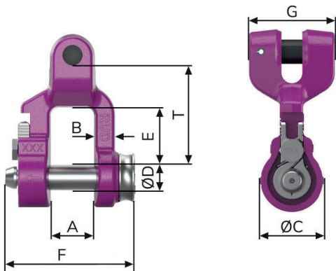
Pic. 28: ICE CCS-FASTLOX 6-16 mm
