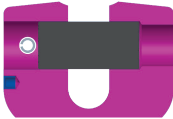
Pic. 9: Assembly of the clevis pin through clamping pin and stepped hole (left). A clevis pin of the next smaller size falls out.
